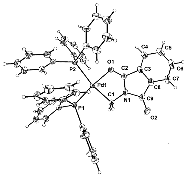
Figure 3. Molecular structure of 14 in the crystal; selected bond lengths (Å) and bond angles (°): Pd(1)–C(1) 2.066(4), N(1)–C(1) 1.454(6), O(2)–C(9) 1.194(6), Pd(1)–P(1) 2.2194(12), N(1)–C(2) 1.341(6), C(2)–C(3) 1.480(6), Pd(1)–P(2) 2.3882(12), N(1)–C(9) 1.429(6), C(8)–C(9) 1.474(8), Pd(1)–O(1) 2.125(3), O(1)–C(2) 1.232(5); C(1)–Pd(1)–O(1) 83.05(15), C(2)–O(1)–Pd(1) 108.0(3), N(1)–C(2)–C(3) 108.9(4), O(1)–Pd(1)–P(2) 87.12(9), C(2)–N(1)–C(9) 111.0(4), O(1)–C(2)–C(3) 127.7(4), C(1)–Pd(1)–P(1) 91.08(13), C(9)–N(1)–C(1) 127.7(4), O(2)–C(9)–C(8) 130.6(5), P(1)–Pd(1)–P(2) 98.50(4), C(2)–N(1)–C(1) 121.0(3), N(1)–C(9)–C(8) 105.0(4), N(1)–C(1)–Pd(1) 103.5(3), O(1)–C(2)–N(1) 123.4(4), O(2)–C(9)–N(1) 124.5(5).
