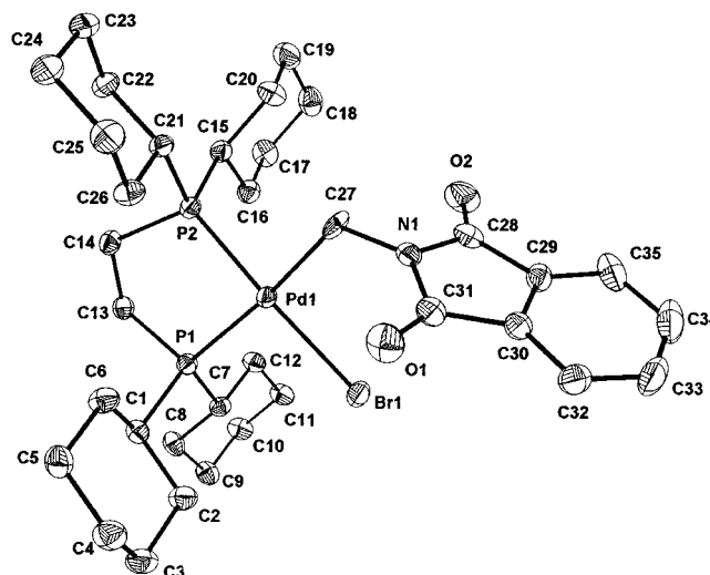
Figure 2. Molecular structure of 11 in the crystal; selected bond lengths (Å) and bond angles ( ^\circ ): Pd(1)–C(27) 2.160(5), N(1)–C(31) 1.402(6), Pd(1)–P(1) 2.3197(13), O(1)–C(31) 1.210(6), Pd(1)–P(2) 2.2324(13), O(2)–C(28) 1.207(6), Pd(1)–Br(1) 2.5068(6), C(28)–C(29) 1.500(7), N(1)–C(27) 1.402(5), C(29)–C(30) 1.365(7), N(1)–C(28) 1.379(6), C(30)–C(31) 1.490(7), C(27)–Pd(1)–P(2) 89.03(12), C(31)–N(1)–C(27) 127.9(5), P(2)–Pd(1)–P(1) 86.66(5), O(1)–C(31)–N(1) 124.8(5), C(27)–Pd(1)–Br(1) 94.32(11), N(1)–C(31)–C(30) 106.3(5), P(1)–Pd(1)–Br(1) 91.25(4), O(1)–C(31)–C(30) 128.9(5), N(1)–C(27)–Pd(1) 115.3(3), O(2)–C(28)–N(1) 124.9(5), C(28)–N(1)–C(27) 121.0(5), N(1)–C(28)–C(29) 106.7(5), C(28)–N(1)–C(31) 110.9(4), O(2)–C(28)–C(29) 128.4(6).
