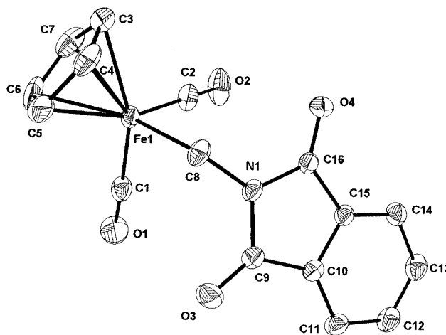
Figure 1. Molecular structure of 2 in the crystal; selected bond lengths (Å) and bond angles (°): Fe(1)–C(1) 1.755(3), O(3)–C(9) 1.204(3), Fe(1)–C(2) 1.750(3), O(4)–C(16) 1.208(3), Fe(1)–C(8) 2.042(3), N(1)–C(8) 1.450(3), O(1)–C(1) 1.144(3), N(1)–C(9) 1.395(3), O(2)–C(2) 1.140(3), N(1)–C(16) 1.391(3); C(2)–Fe(1)–C(1) 93.71(14), O(1)–C(1)–Fe(1) 176.0(3), C(1)–Fe(1)–C(8) 92.77(12), O(2)–C(2)–Fe(1) 177.3(3), C(2)–Fe(1)–C(8) 92.07(12), N(1)–C(8)–Fe(1) 119.7(2), C(16)–N(1)–C(9) 111.4(2), O(3)–C(9)–N(1) 124.9(2), C(16)–N(1)–C(8) 124.1(2), O(4)–C(16)–N(1) 124.6(2), C(9)–N(1)–C(8) 124.2(2).
