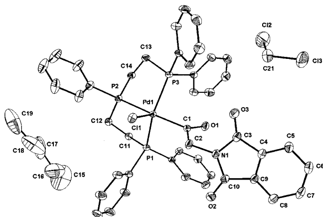
Figure 5. Molecular structure of 16 in the crystal; selected bond lengths (Å) and bond angles (°): Pd(1)–C(1) 2.035(2), Pd(1)–Cl(1) 2.6855(6), C(3)–N(1) 1.399(3), Pd(1)–P(1) 2.3133(6), C(1)–C(2) 1.540(3), N(1)–C(10) 1.379(3), Pd(1)–P(2) 2.3381(6), O(1)–C(1) 1.195(3), O(2)–C(10) 1.214(3), Pd(1)–P(3) 2.3297(6), C(2)–N(1) 1.454(3), O(3)–C(3) 1.195(3); P(1)–Pd(1)–P(2) 85.20(2), C(1)–Pd(1)–P(3) 91.67(6), C(2)–C(1)–Pd(1) 115.07(15) P(1)–Pd(1)–P(3) 137.67(2) P(1)–Pd(1)–Cl(1) 114.10(2) N(1)–C(2)–C(1) 112.64(19) P(3)–Pd(1)–P(2) 85.30(2), P(2)–Pd(1)–Cl(1) 97.626(19) C(10)–N(1)–C(2) 124.8(2), C(1)–Pd(1)–P(1) 89.82(7), P(3)–Pd(1)–Cl(1) 108.02 (2) C(10)–N(1)–C(3) 111.9(2), C(1)–Pd(1)–Cl(1) 93.61(7), O(1)–C(1)–Pd(1) 125.99(17) C(3)–N(1)–C(2) 122.8(2) C(1)–Pd(1)–P(2) 168.76(7) O(1)–C(1)–C(2) 118.9(2)
