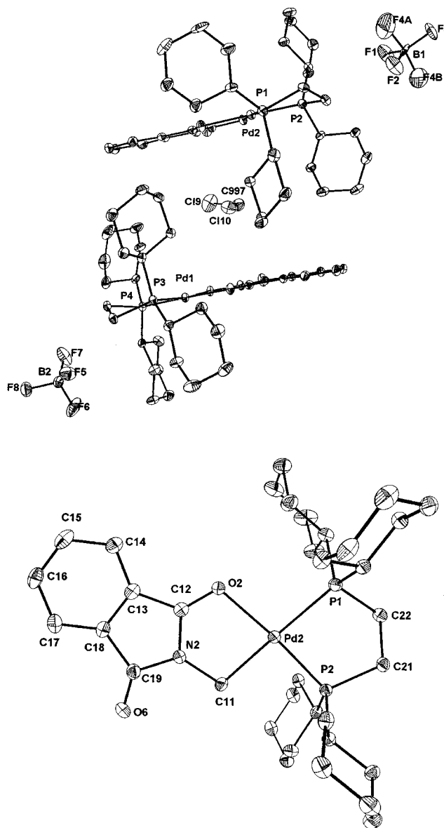
Figure 4. Molecular structure of 15 in the crystal; selected bond lengths (Å) and bond angles (°): Pd(2)–C(11) 2.083(4), N(2)–C(11) 1.464(5), O(6)–C(19) 1.202(5), Pd(2)–P(1) 2.3193(11), N(2)–C(12) 1.364(5), C(12)–C(13) 1.473(5), Pd(2)–P(2) 2.2203(10), N(2)–C(19) 1.403(5), C(18)–C(19) 1.488(6), Pd(2)–O(2) 2.148(3), O(2)–C(12) 1.238(5); C(11)–Pd(2)–O(2) 82.71(12), C(12)–O(2)–Pd(2) 109.4(3), N(2)–C(12)–C(13) 107.6(4), O(2)–Pd(2)–P(1) 98.49(7), C(12)–N(2)–C(19) 111.0(3), O(2)–C(12)–C(13) 129.7(4), C(11)–Pd(2)–P(2) 92.66(11), C(19)–N(2)–C(11) 127.7(3), O(6)–C(19)–C(18) 129.7(4), P(1)–Pd(2)–P(2) 86.12(4), C(12)–N(2)–C(11) 121.1(3), N(2)–C(19)–C(18) 105.9(4), N(2)–C(11)–Pd(2) 104.2(2), O(2)–C(12)–N(2) 122.6(4), O(6)–C(19)–N(2) 124.4(4).
